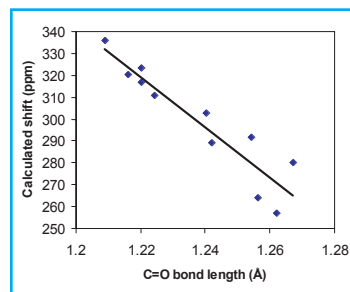
▲ Figure 2. Calculated 17 O isotropic chemical shift vs. C=O bond length
