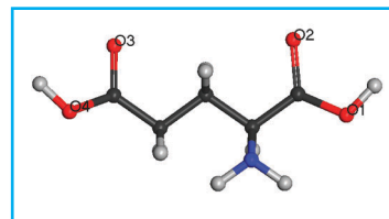
▲ Figure 1. Glutamic acid molecule illustrating naming convention for O-atoms
