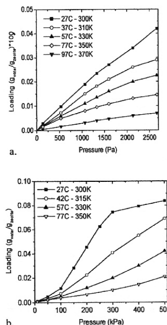
Figure 1. a. Water adsorption isotherms in defect-free silicalite from 300 to 370 K at low pressures and b. from 300 to 350 K at high pressures.
